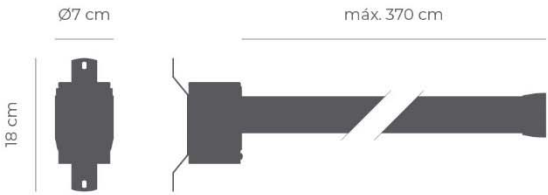
Mural BASIC Vertical Esc. 1:10 (Peso: 1Kg)
